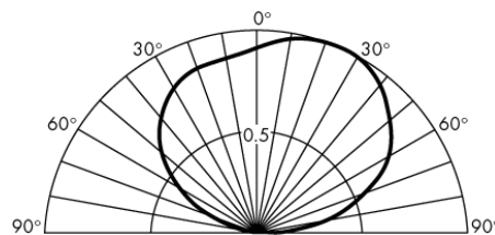
Spatial distribution of the 950nm infrared LED
